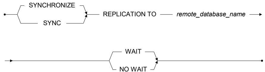
Figure 17-8 Syntax for the SYNCHRONIZE REPLICATION Statement
