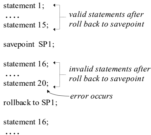
Figure 9-2 Using Savepoints
