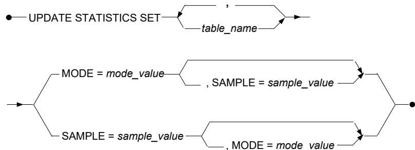
Figure 20-2 Syntax for the UPDATE STATISTICS SET statement
