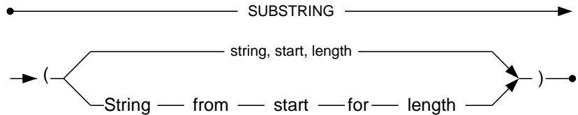
Figure 4-125 SUBSTRING syntax
