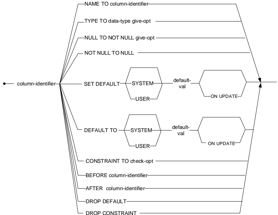
Figure 3-20 ATTRIBUTE-MODIFY-COLUMN-DEF syntax
