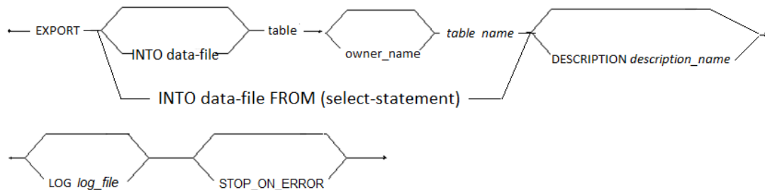
Figure 6-6 EXPORT syntax
