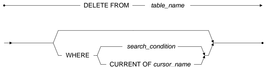
Figure 3-71 DELETE syntax
