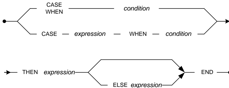
Figure 3-120 CASE Syntax
