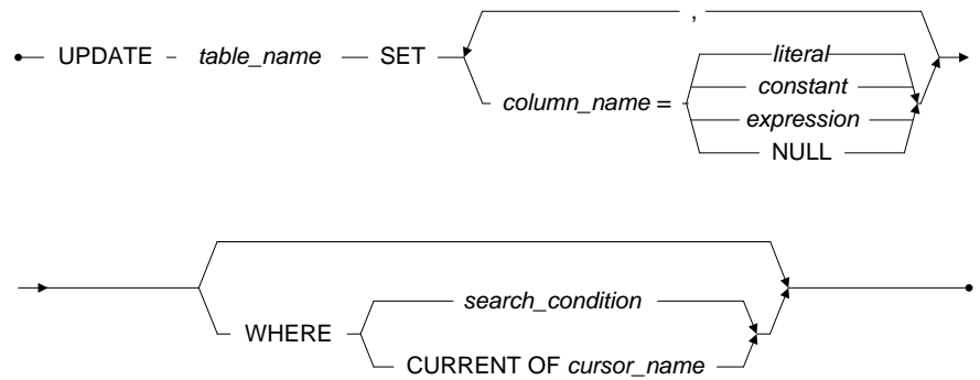
Figure 3-153 UPDATE syntax
