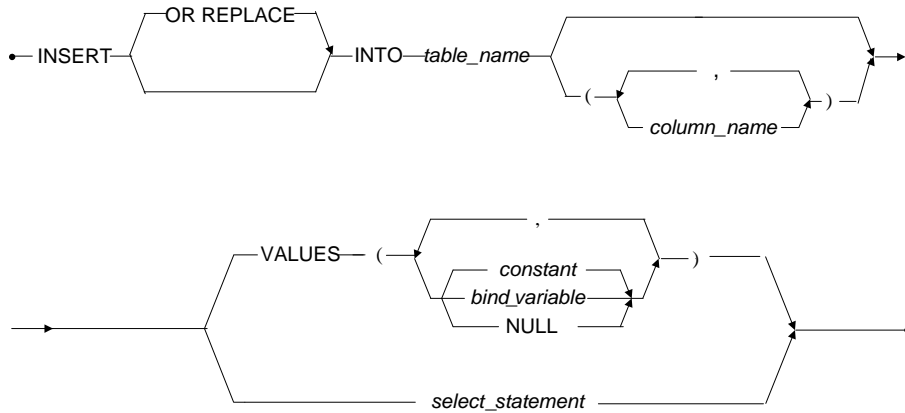
Figure 3-93 INSERT syntax
