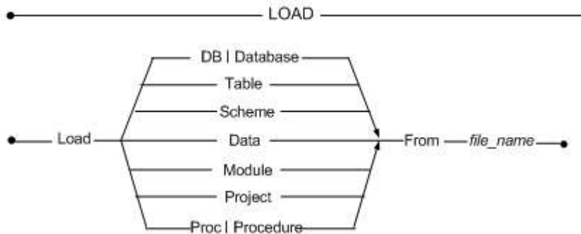
Figure 6-8 LOAD syntax
