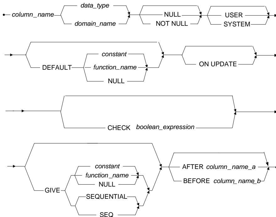
Figure 3-22 COLUMN_DEFINITIONS syntax
