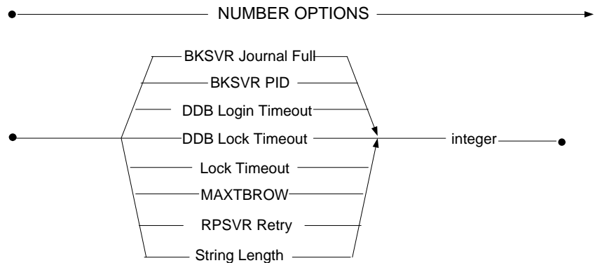
Figure 3-142 Number Options syntax
