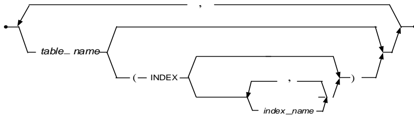
Figure 3-155 UPDATE STATISTICS Object List syntax
