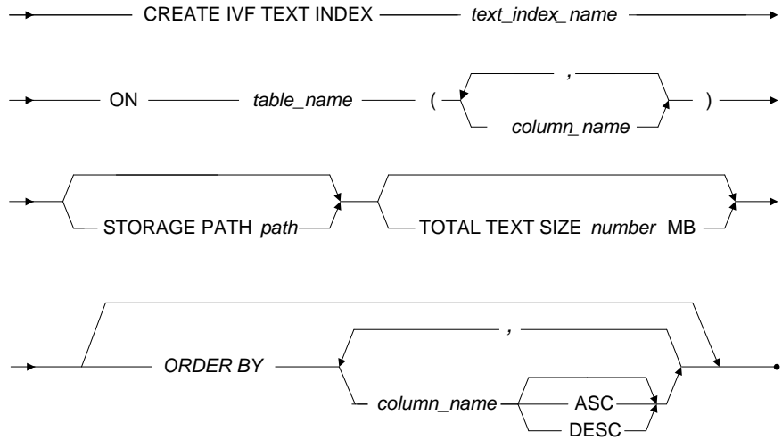
Figure 3-66 CREATE IVF TEXT INDEX syntax
