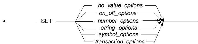
Figure 3-138 SET CONNECTION OPTIONS syntax
