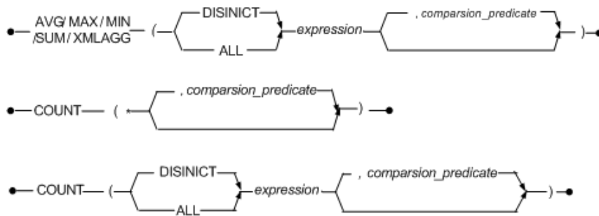
Figure 3-136 AGGREGATE FUNCTION syntax
