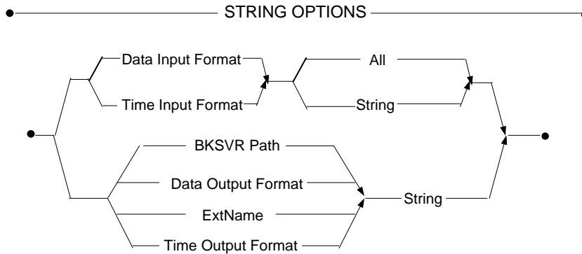
Figure 3-143 String Options syntax
