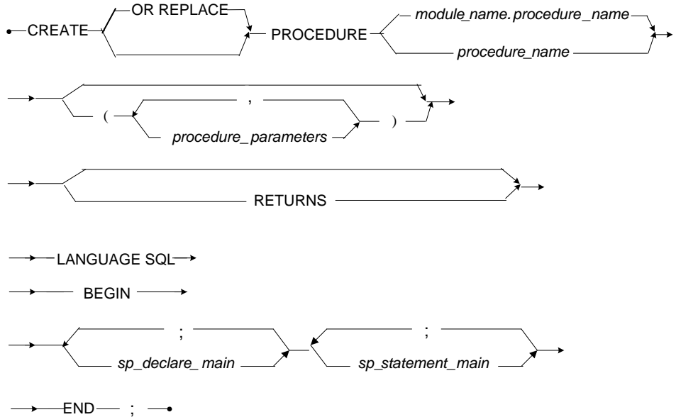
Figure 3-53 CREATE SQL SP syntax
