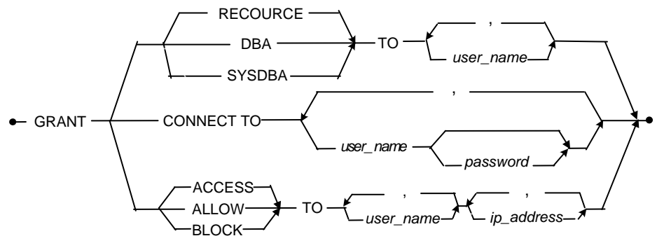
Figure 3-92 GRANT (Security Privileges) syntax
