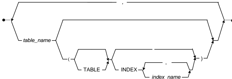
Figure 3-152 UNLOAD STATISTICS Object List syntax
