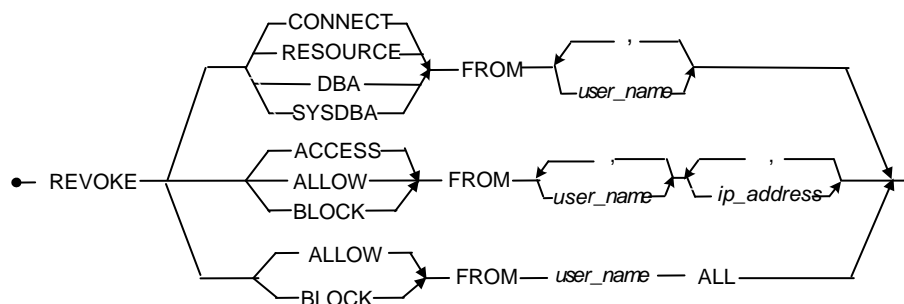
Figure 3-106 REVOKE (Security Privileges) syntax
