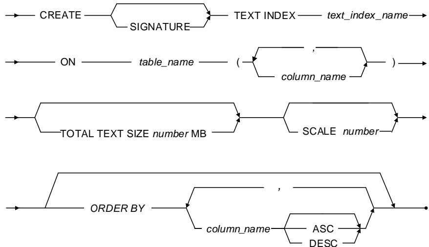
Figure 3-65 CREATE SIGNATURE TEXT INDEX syntax
