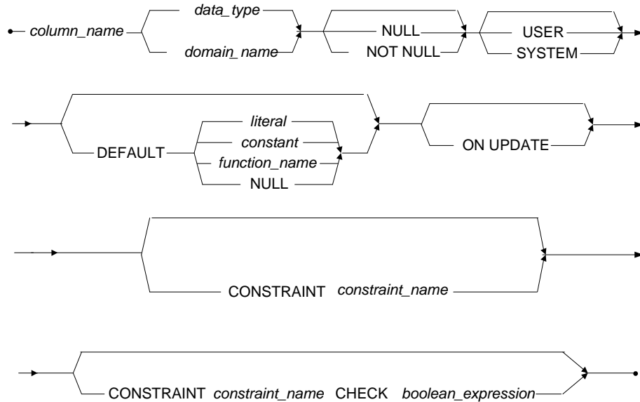
Figure 3-61 Column Definitions syntax
