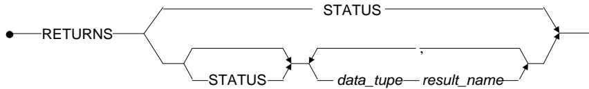
Figure 3-51 CREATE PROCEDURE: procedure_return_result syntax
