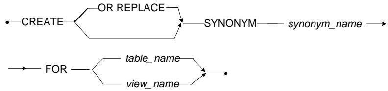
Figure 3-57 CREATE SYNONYM syntax
