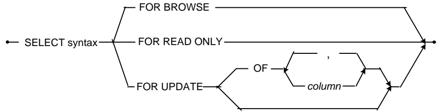
Figure 3-134 FOR BROWSE Clause syntax
