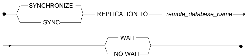
Figure 3-150 SYNCHRONIZE SCHEDULE syntax
