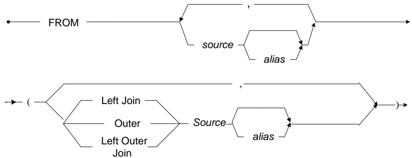
Figure 3-126 DBMaker Outer-Join Syntax
