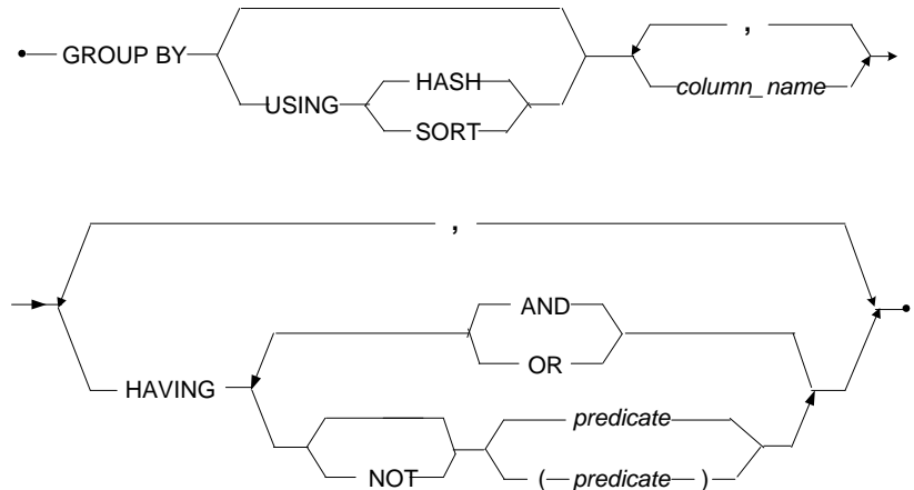
Figure 3-131 GROUP BY Clause syntax
