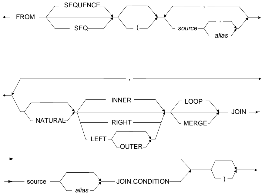
Figure 3-124 ANSI Join syntax
