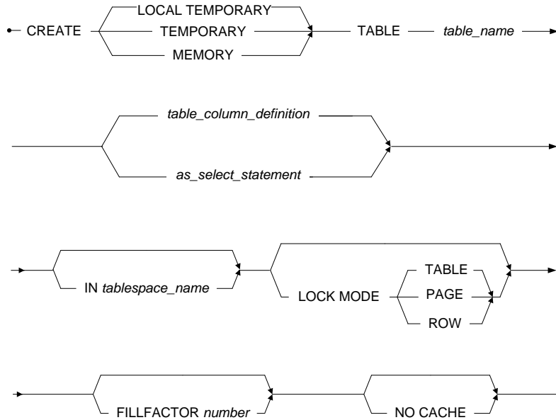
Figure 3-58 CREATE TABLE syntax
