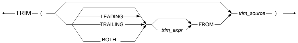
Figure 4-118 TRIM function syntax
