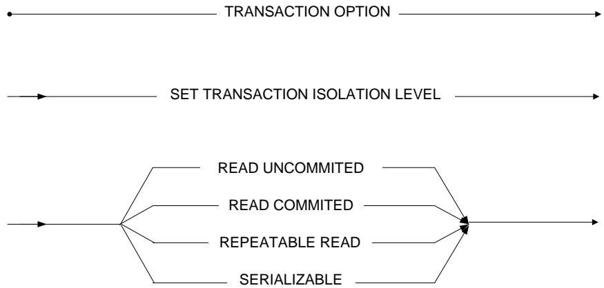
Figure 3-145 TRANSACTION OPTIONS syntax
