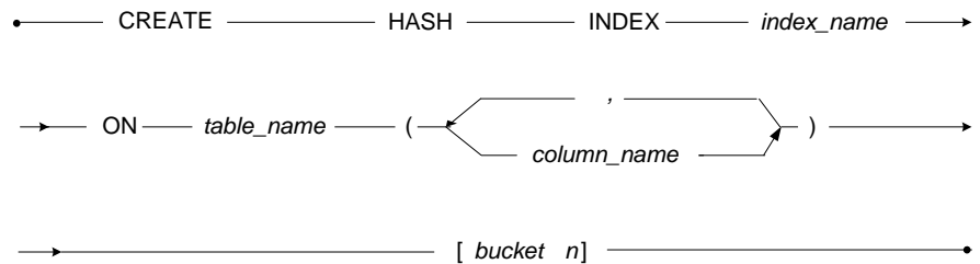
Figure 3-46 CREATE HASH INDEX syntax
