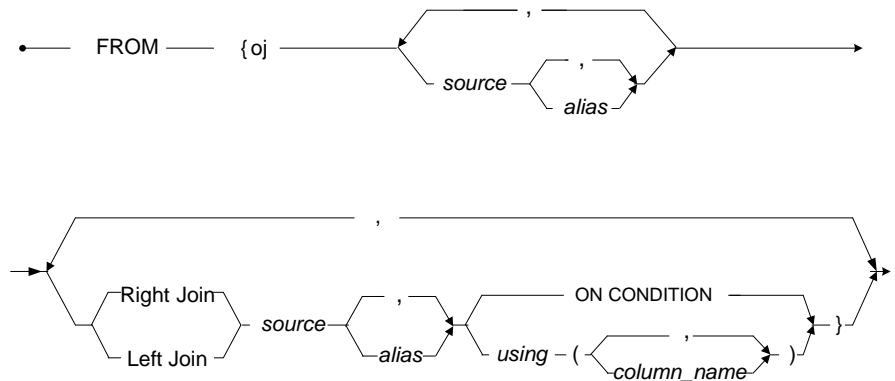
Figure 3-127 ODBC Outer-Join Syntax
