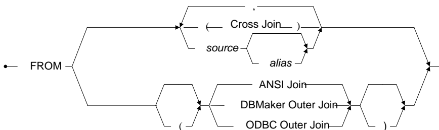
Figure 3-112 FROM Clause syntax
