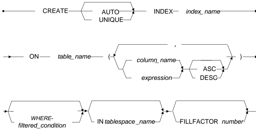
Figure 3-47 CREATE INDEX syntax
