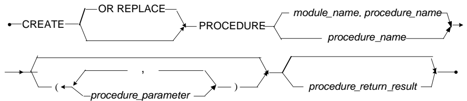
Figure 3-49 CREATE PROCEDURE syntax
