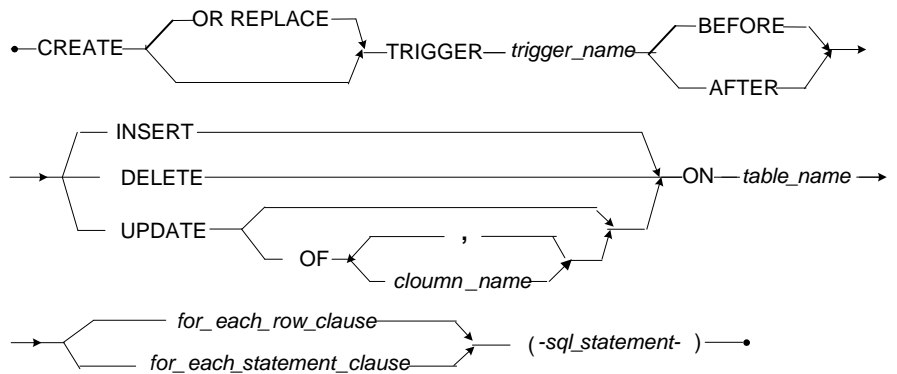
Figure 3-67 CREATE TRIGGER syntax
