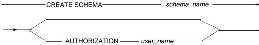
Figure 3-56 CREATE SCHEMA syntax
