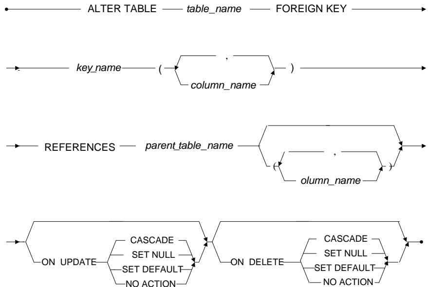
Figure 3-18 ALTER TABLE FOREIGN KEY syntax
