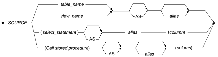
Figure 3-113 SOURCE subclause syntax
