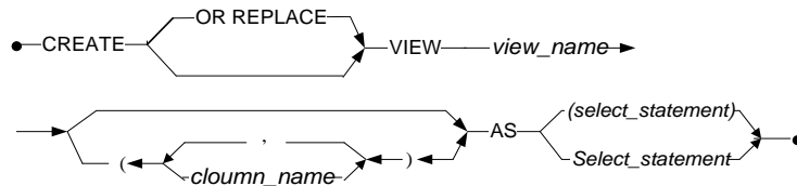
Figure 3-70 CREATE VIEW syntax
