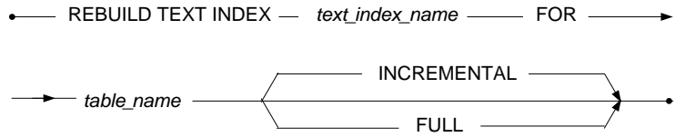
Figure 3-100 REBUILD TEXT INDEX syntax
