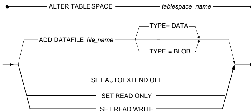
Figure 3-30 ALTER TABLESPACE syntax
