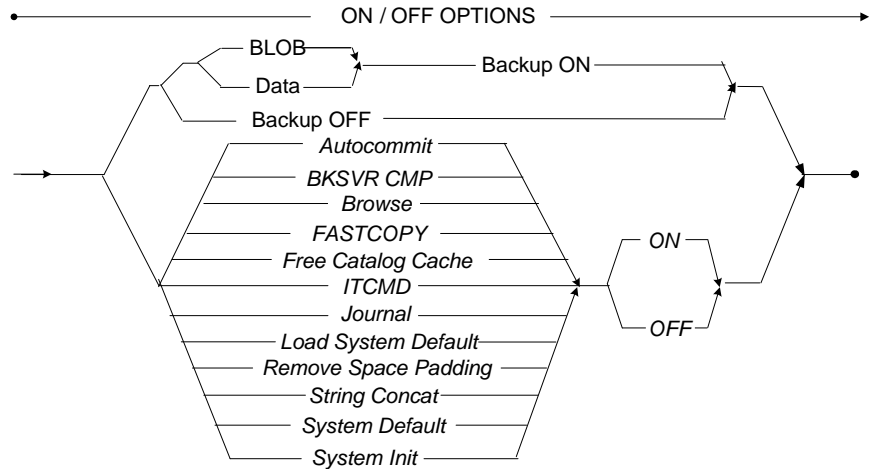
Figure 3-140 ON/OFF Options syntax
