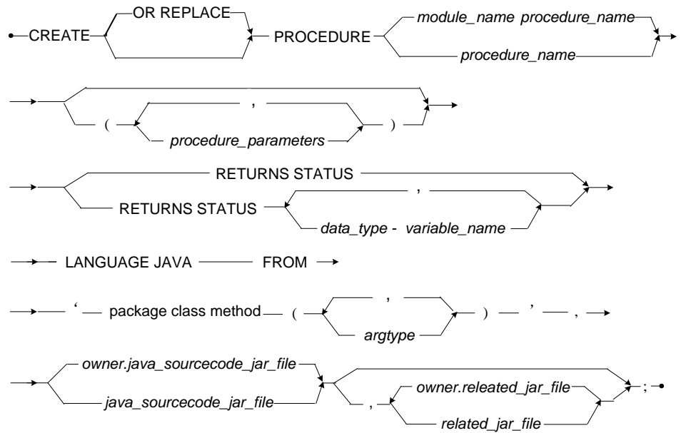
Figure 3-52 CREATE JavaSP syntax
