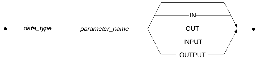
Figure 3-50 CREATE PROCEDURE: procedure_paramter syntax
