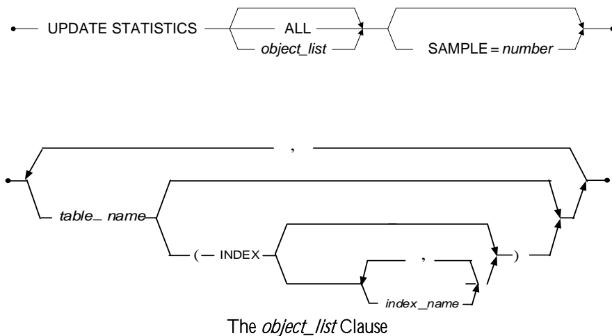
Figure 19-1 Syntax for the UPDATE STATISTICS Statement
