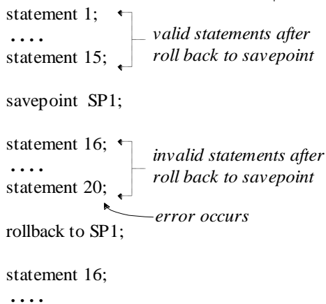
Figure 9-2 Using Savepoints
